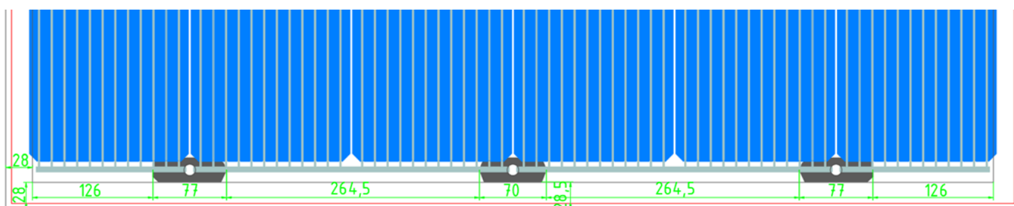
Figure 10 Position of the junction box in SOLID Series module
