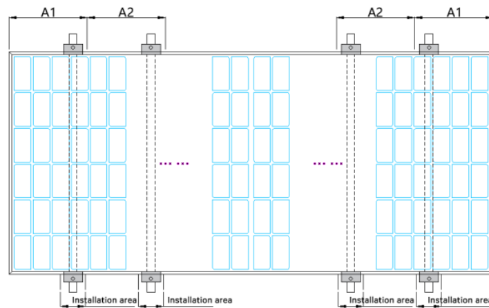
Figure 12: clamps fixed method in long side
