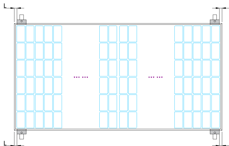
Figure 11: clamps fixed method in long side
